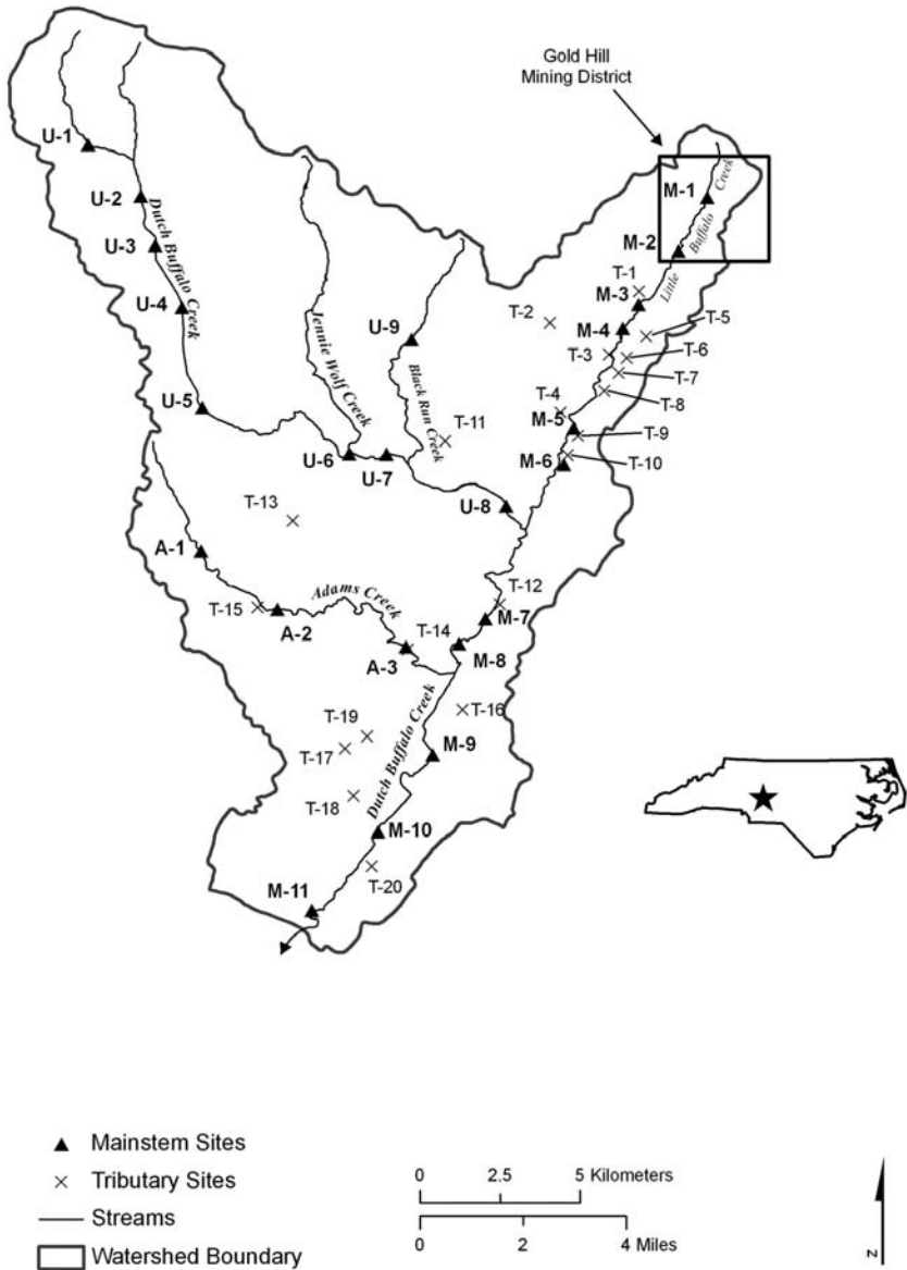
Figure 1. Study area map with sampling site locations where “M” refers to main stem contaminated sites and “T” refers to background tributary sites. Sites with “A” and “U” were also visited but the results are not included in this study.
