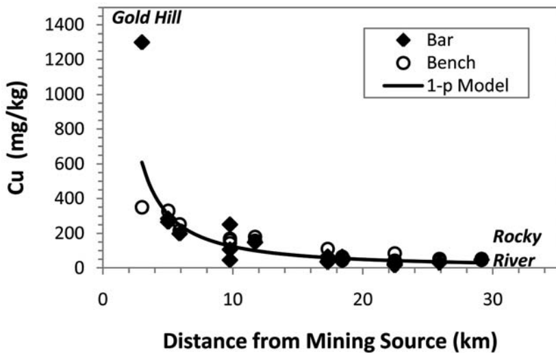
Figure 3. Longitudinal trends in contamination of sediments by Cu. The one-parameter spatial regression model for all-combined samples is shown as the curve for Log Cu over Log distance (Table 4).
