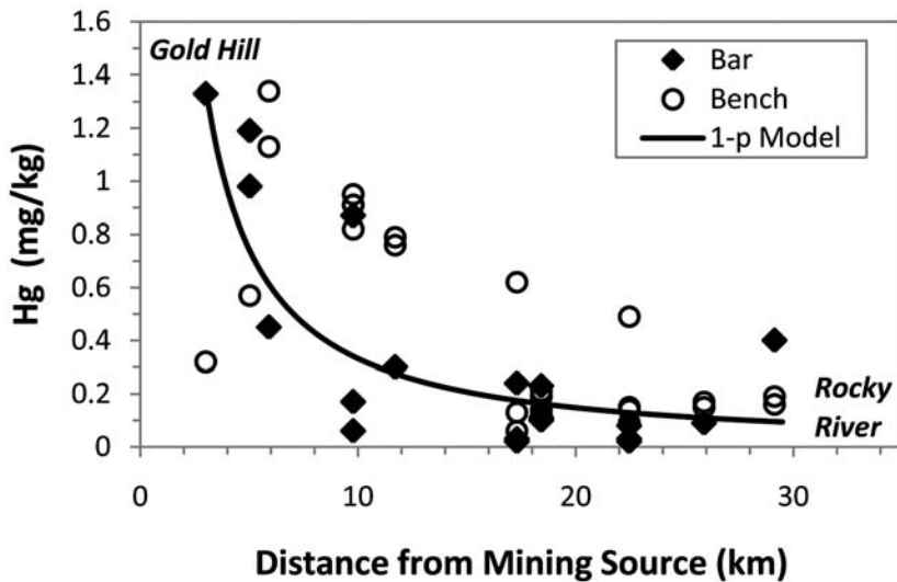
Figure 2. Longitudinal trends in contamination of sediments by Hg. The one-parameter spatial regression model for all-combined samples is shown as the curve for Log Hg over Log distance (Table 4).
