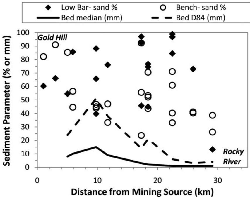
Figure 4. Downstream trends in sediment parameters.
